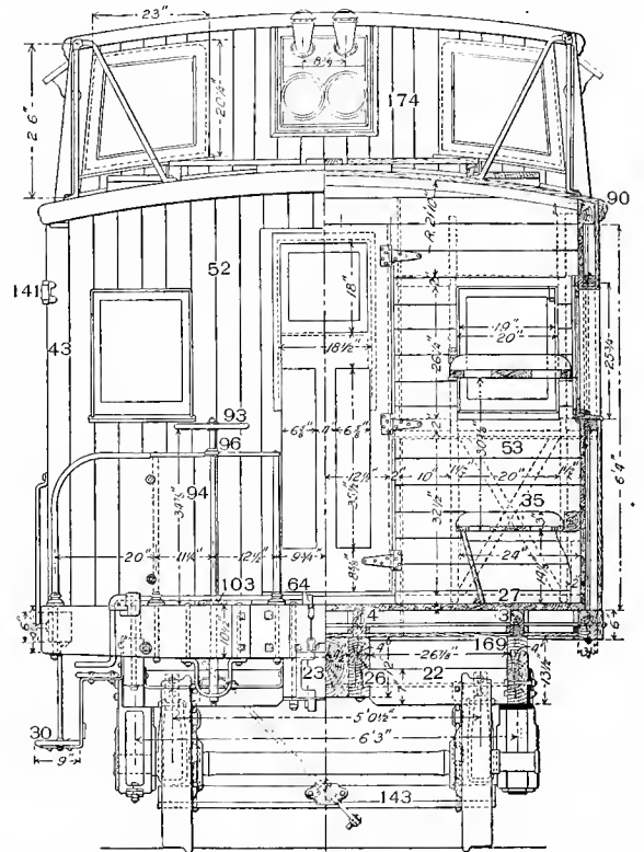
Fig. 388. Half End Elevation and Half Cross Section.
